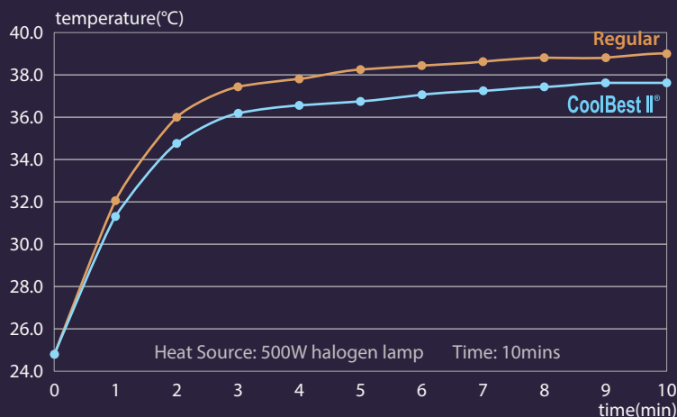
Comparison of the temperature rising curve
